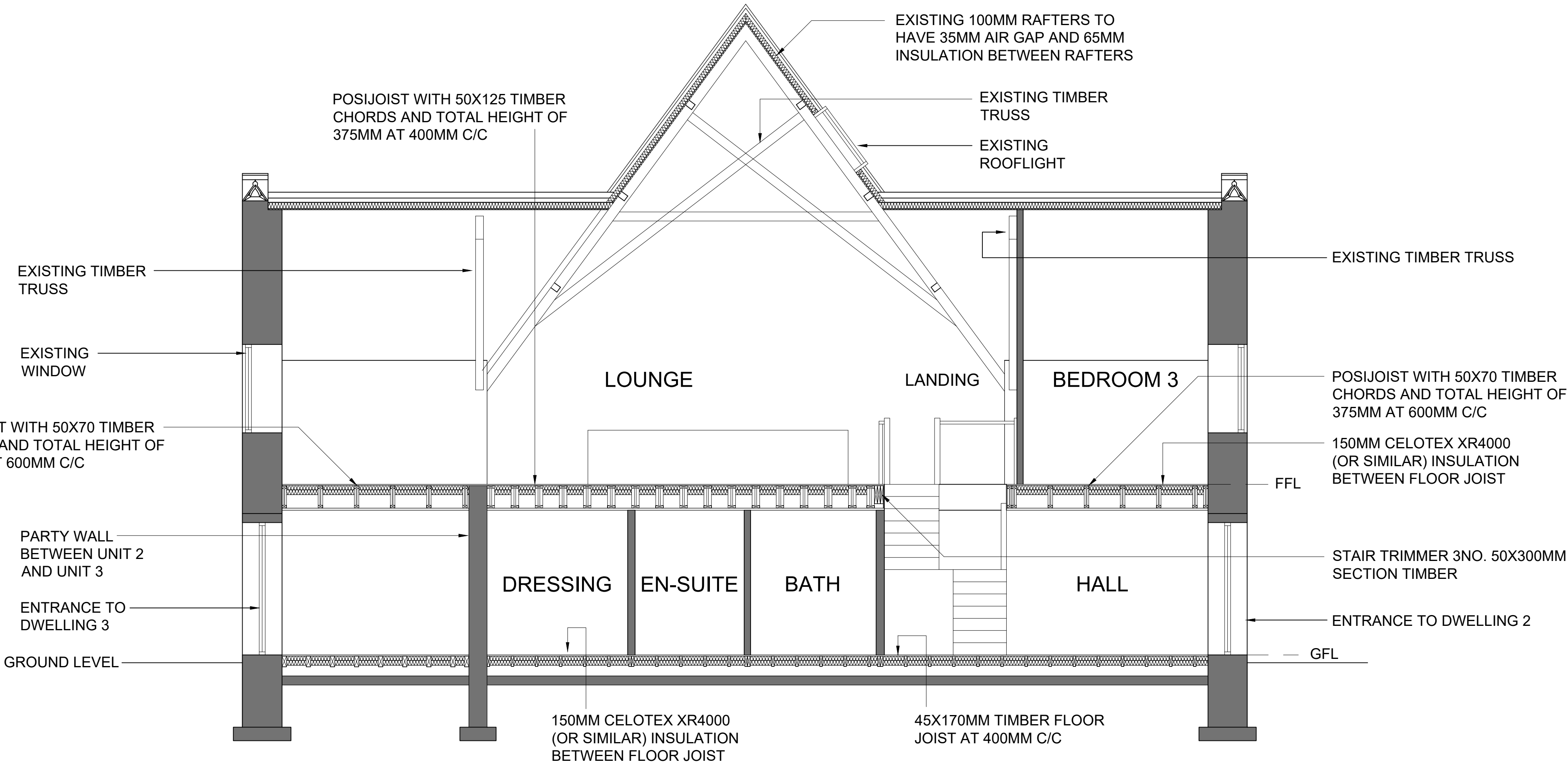
PROPOSED SECTION B-B
