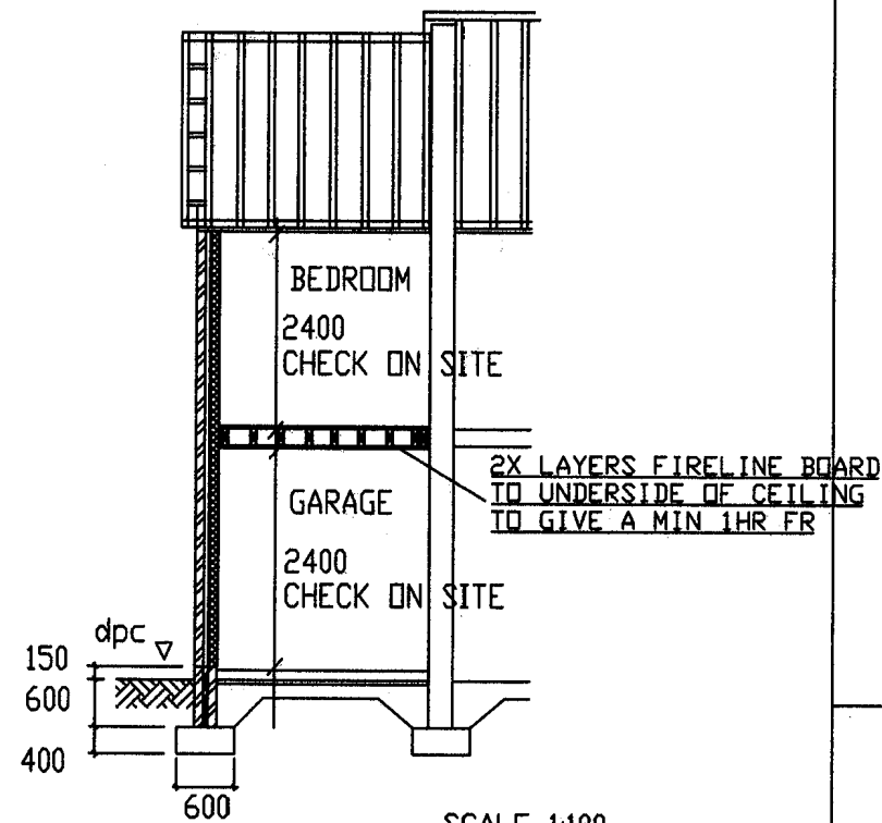
SCALE 1:100 TYPICAL SECTION THRO ON EXTENSION
