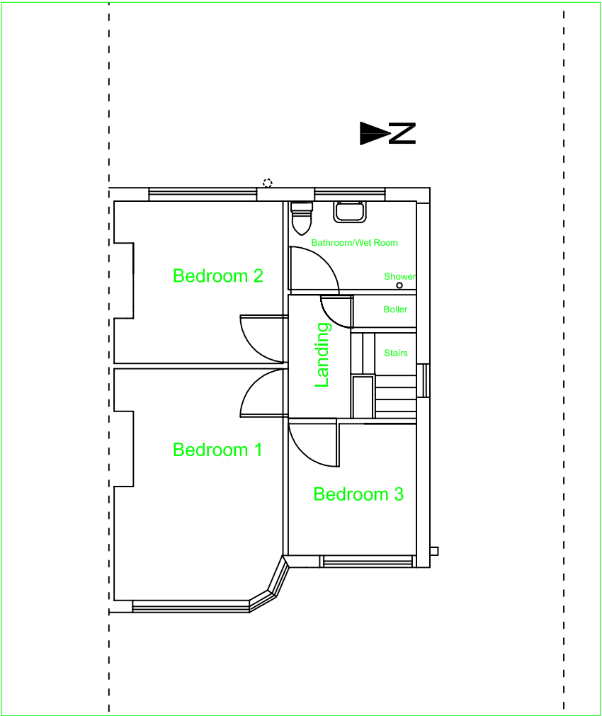
Existing First Floor Layout
