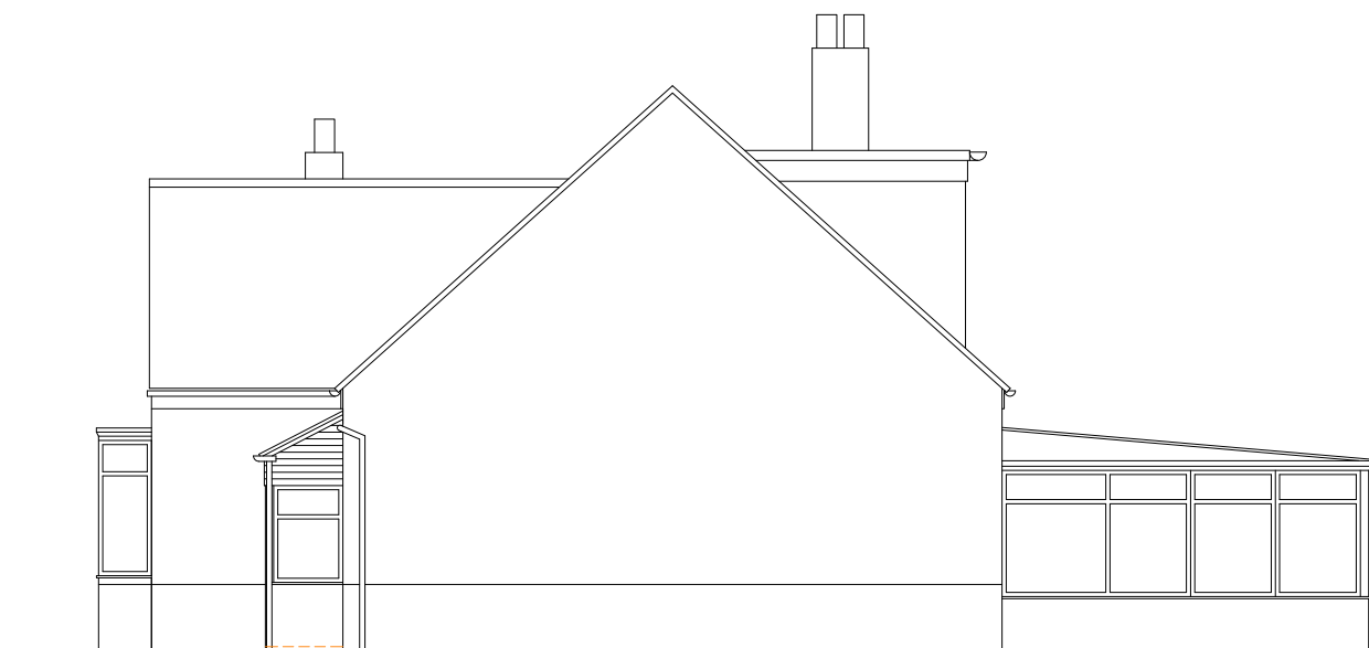
EXISTING SIDE ELEVATION (NW)
