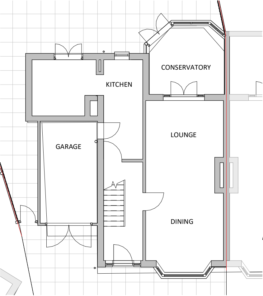
GF PLAN
