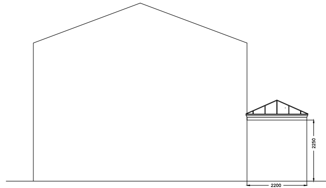
Proposed R/H Elevation
