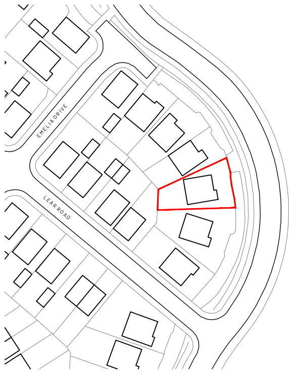
EXISTING LOCATION PLAN SCALE @ 1:1250
