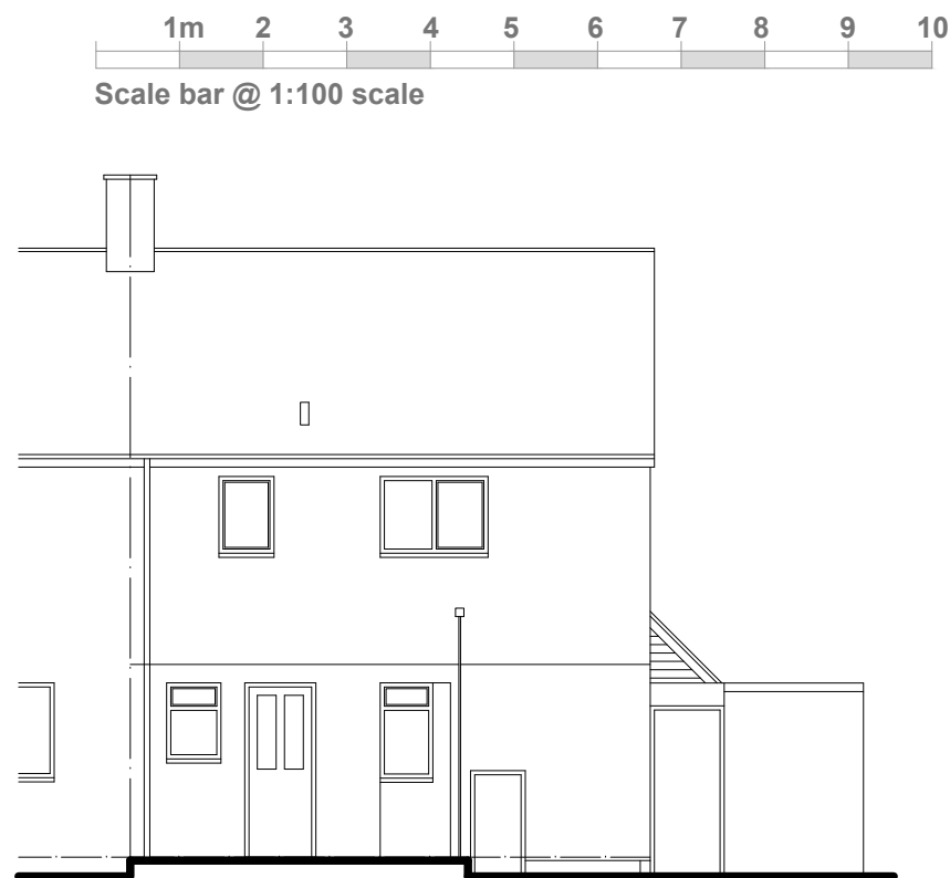
Existing rear elevation @ 1:100 scale
