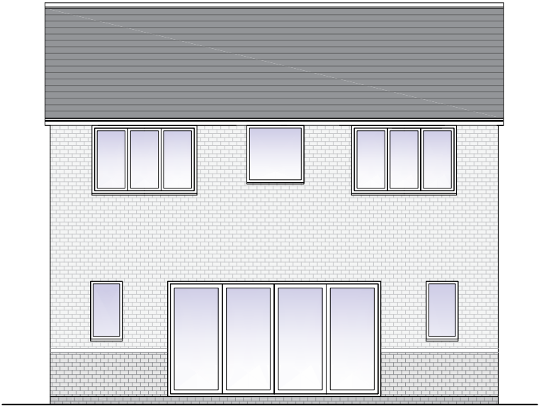
EXISTING REAR ELEVATION (Scale 1:100) SCALE BAR - (mm) 500 1000 2000
