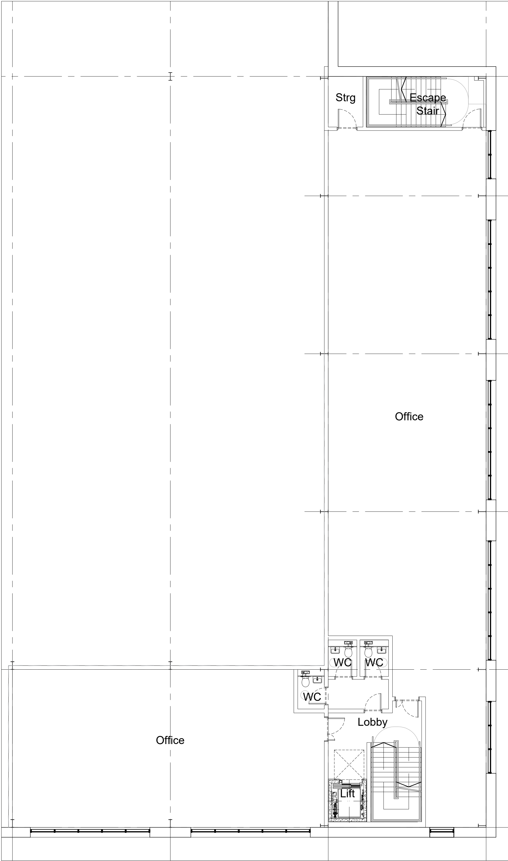
02 Unit 03 GA FF Office Plan 1:100@A1 / 1:200@A3
