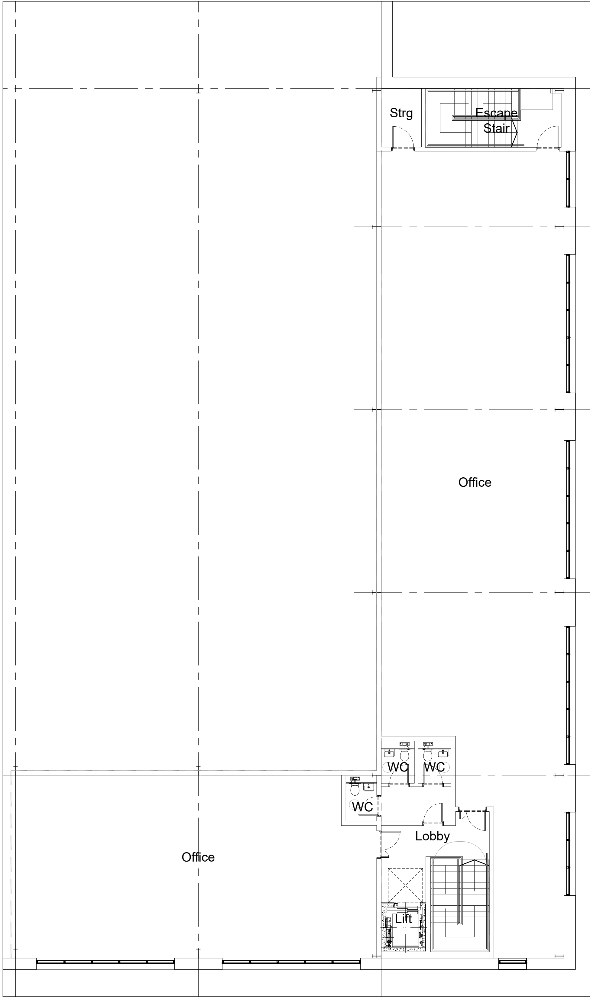
03 Unit 03 GA SF Office Plan 1:100@A1 / 1:200@A3
