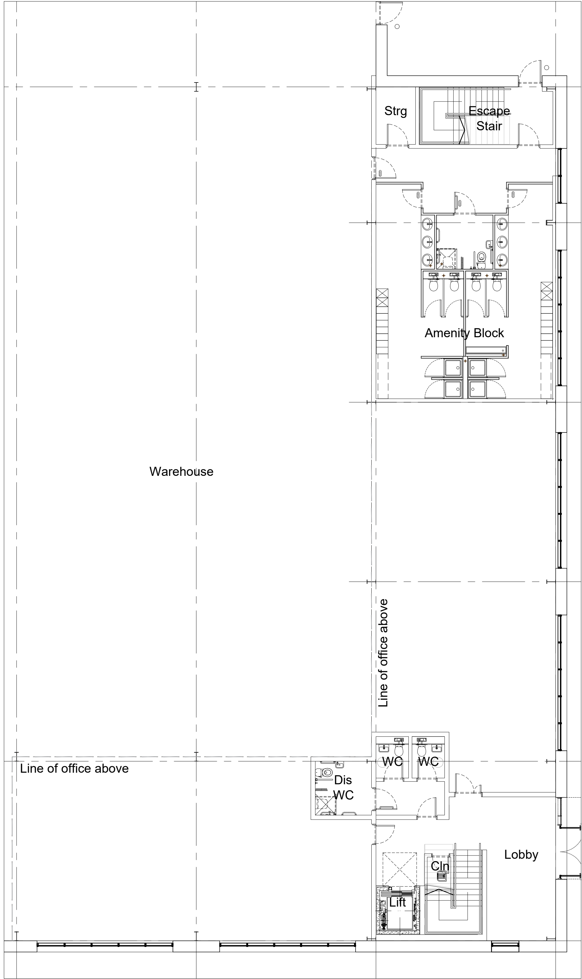
01 Unit 03 GA GF Main Entrance Plan 1:100@A1 / 1:200@A3
