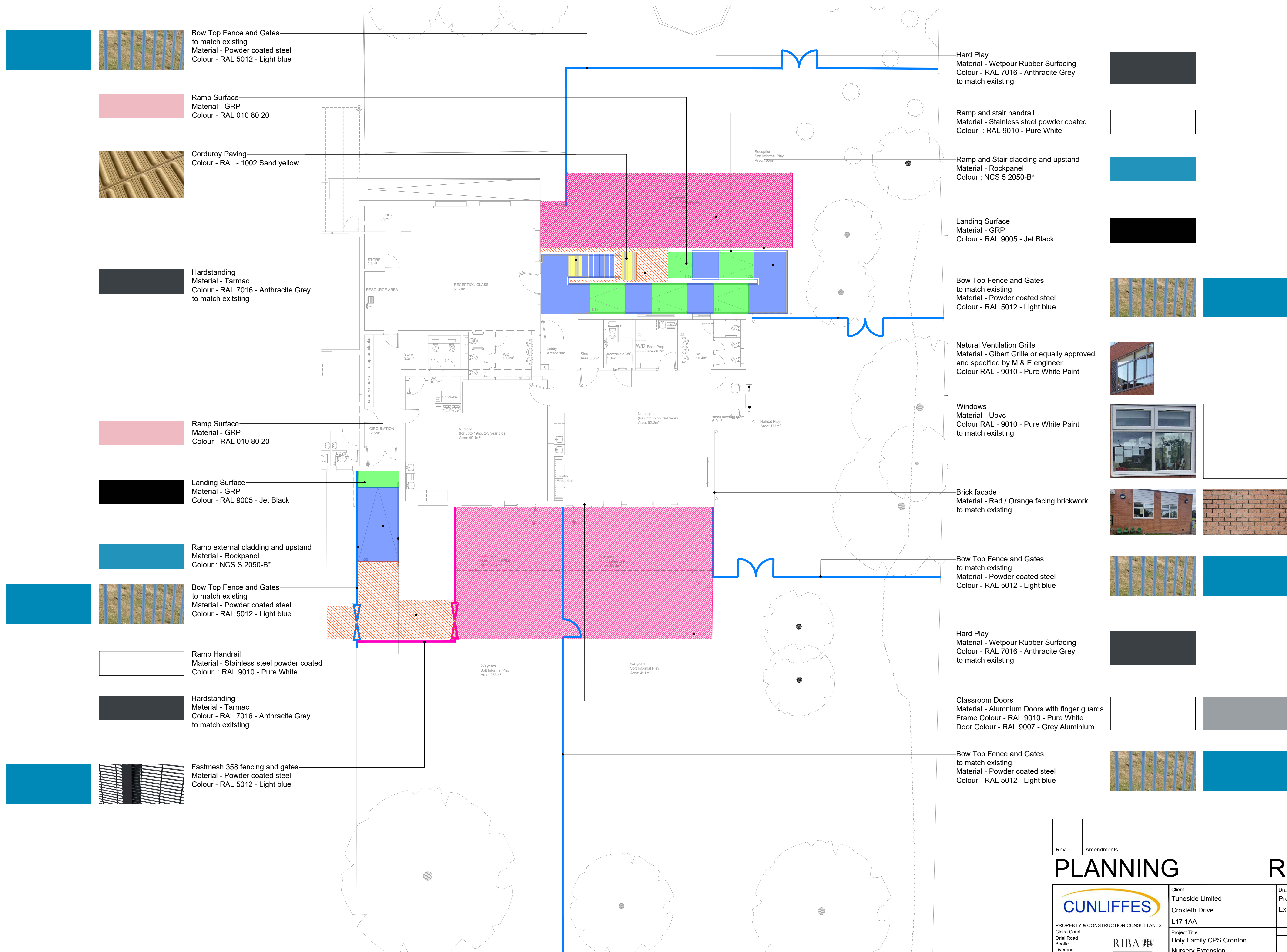
Proposed Materials Ground Floor Layout Plan Scale 1:100
