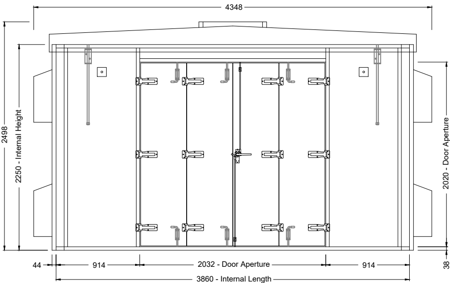
FRONT & REAR ELEVATIONS
