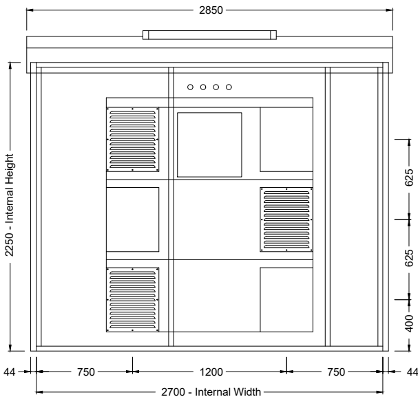
RH & LH SIDE ELEVATIONS
