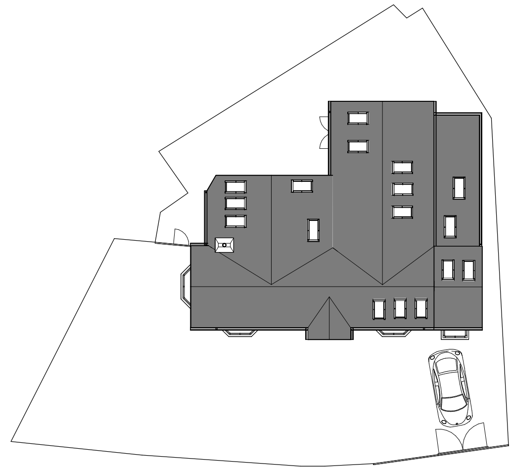
1 Site Layout Proposed 1 : 200
