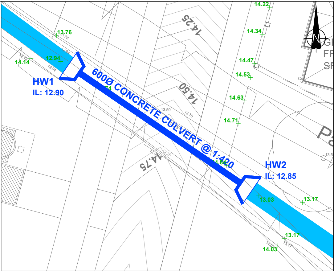
LAYOUT PLAN - SCALE 1:250
