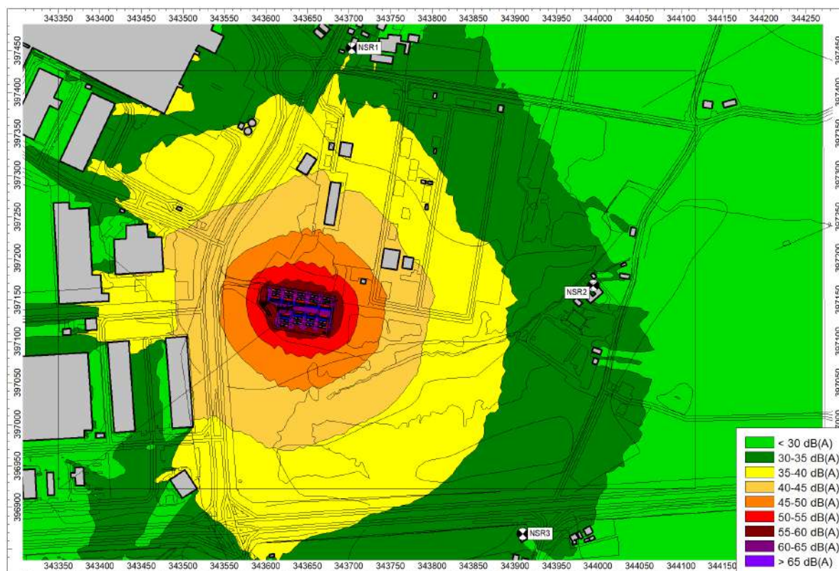
FIGURE 3: SPECIFIC SOUND LEVEL MAP - DAYTIME
