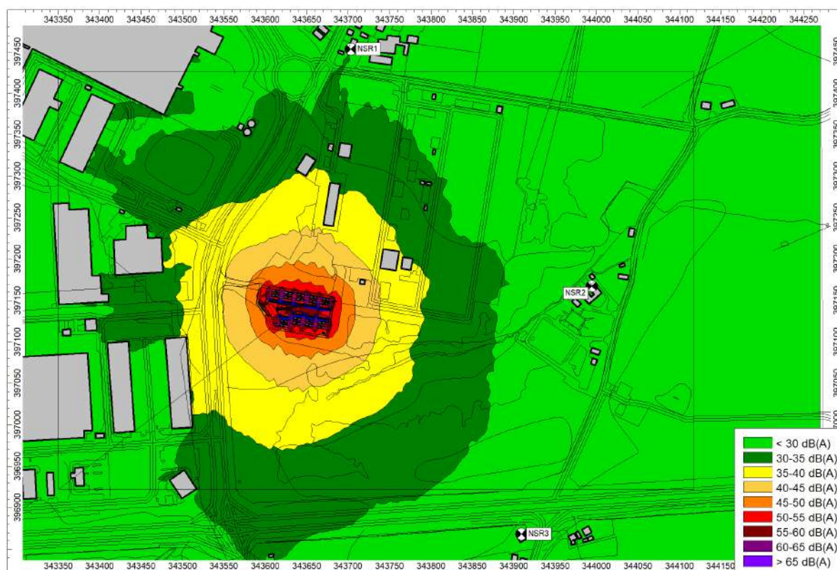
FIGURE 4: SPECIFIC SOUND LEVEL MAP - NIGHT-TIME
