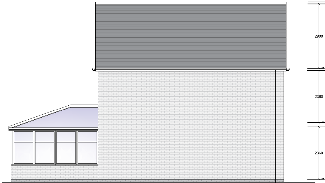
PROPOSED SIDE ELEVATION (Scale 1:100) SCALE BAR - (mm) 2000 1000 500
