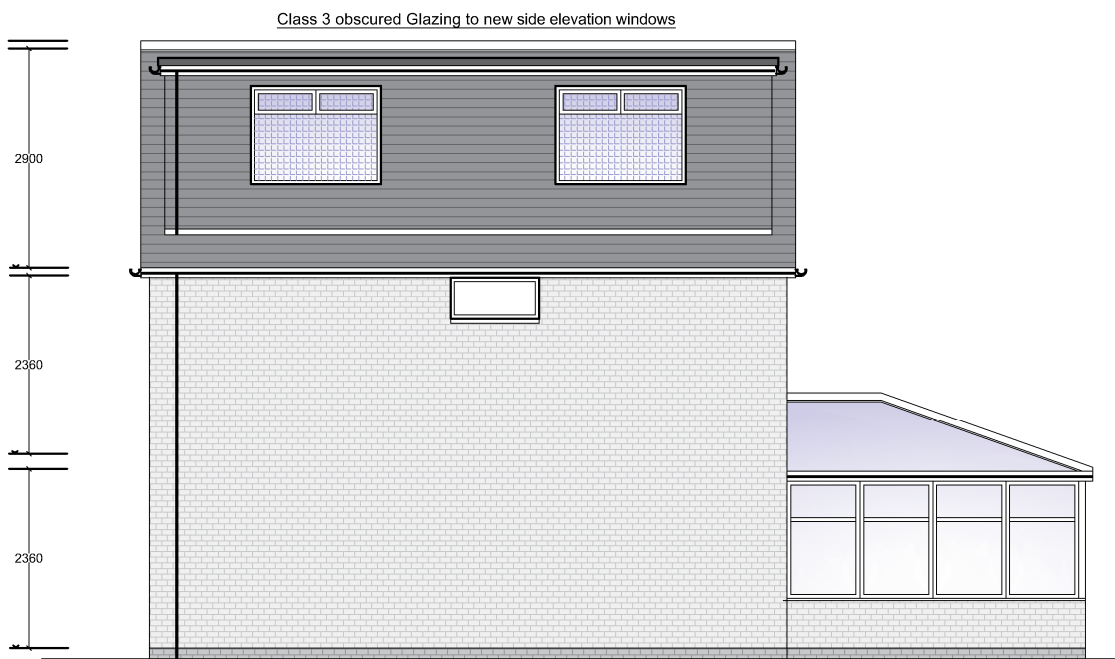
PROPOSED SIDE ELEVATION (Scale 1:100) SCALE BAR - (mm) 500 1000 2000
