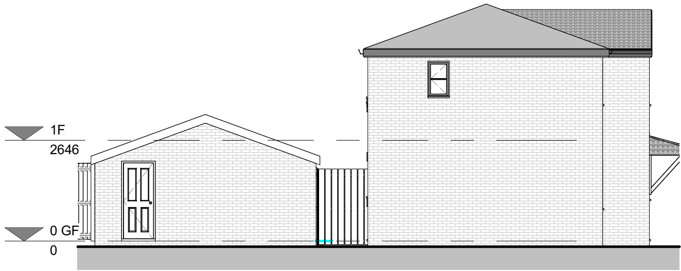
SIDE ELEVATION II 1:100
