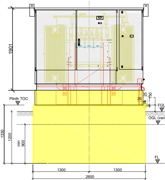
Section 03
