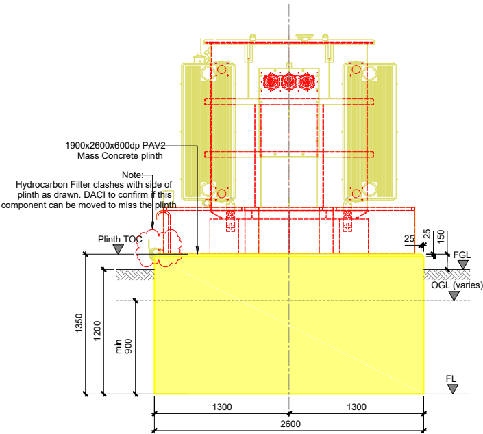
Section 02
