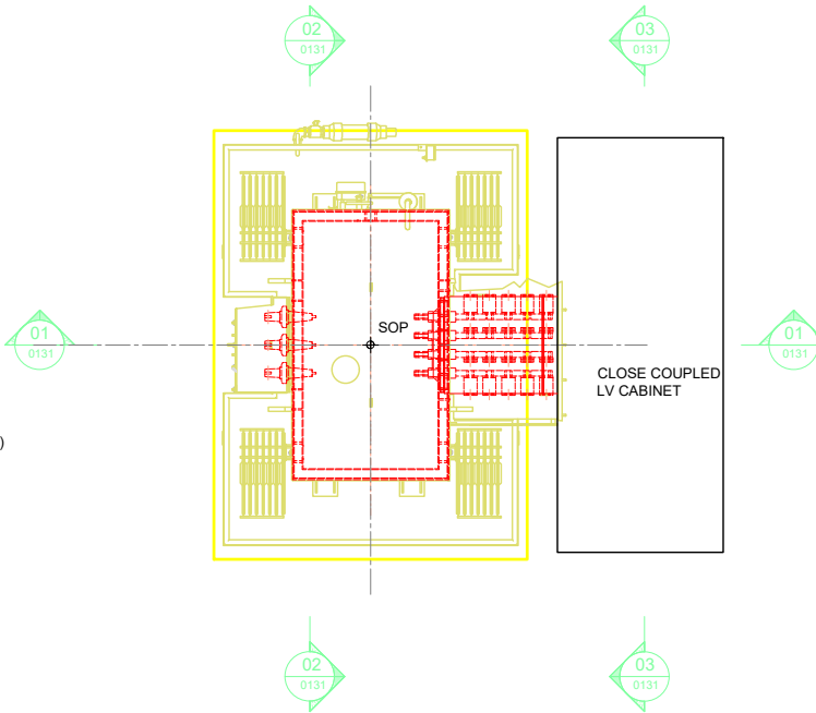
Foundation Plan
