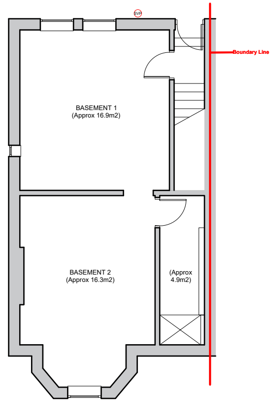
EXISTING BASEMENT FLOOR PLAN Scale - 1:100
