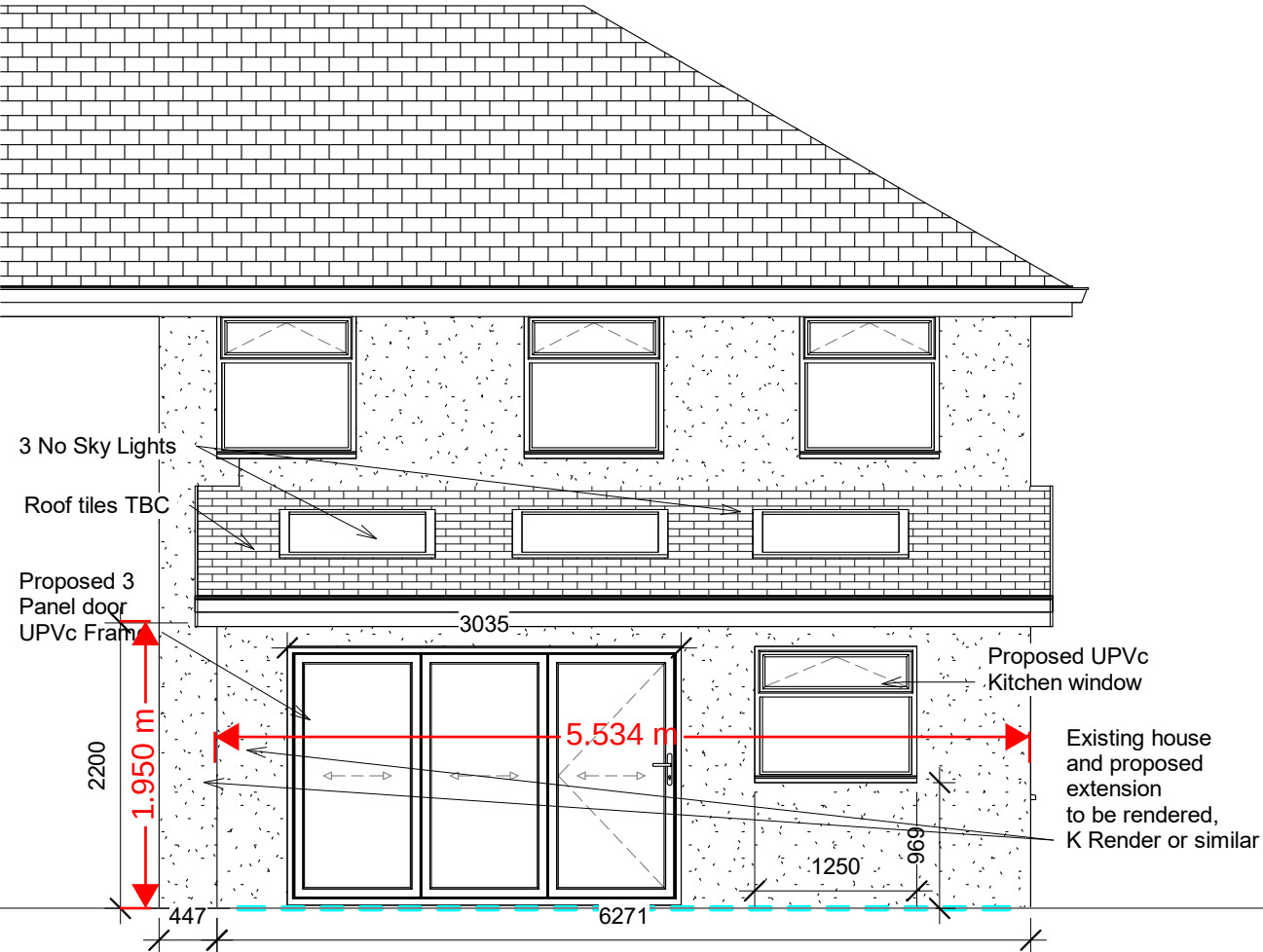
Rear Elevation 1 : 50
