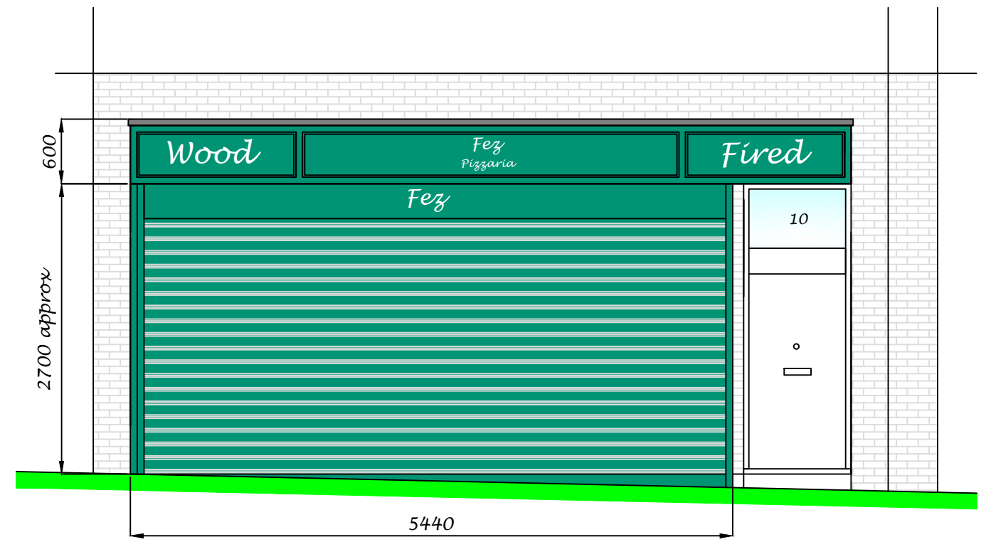
Proposed Shutter Elevation
