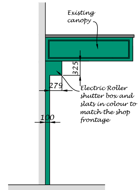
Proposed Shutter Elevation
