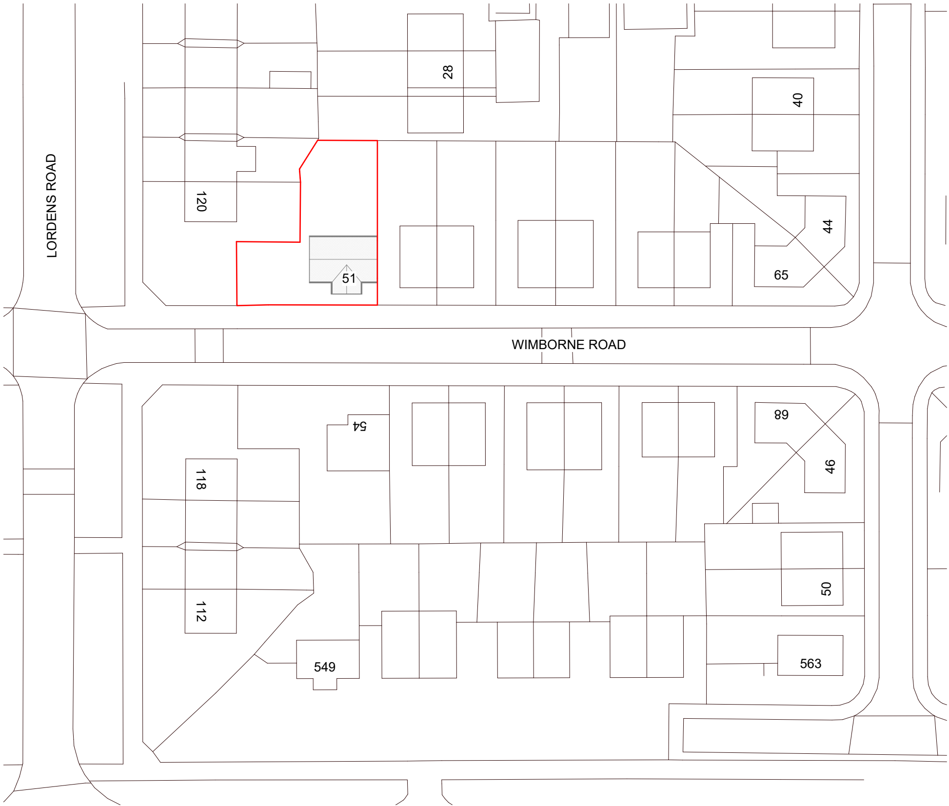
Location Plan 1 : 500
