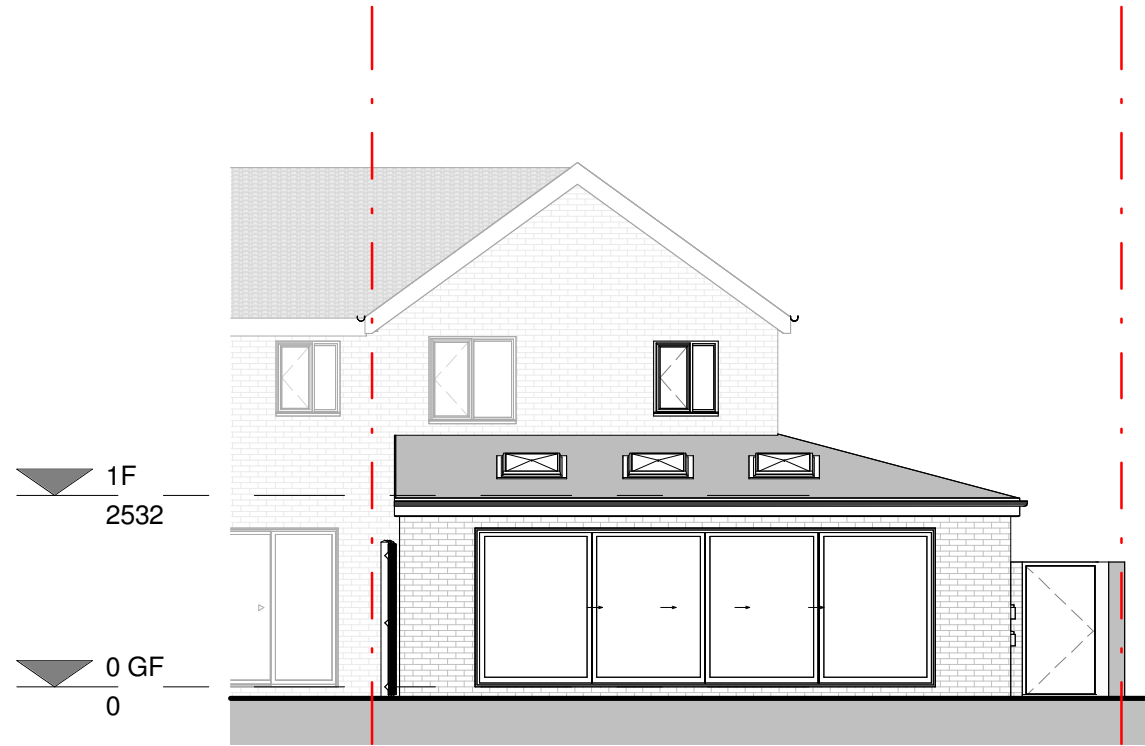
FRONT ELEVATION
