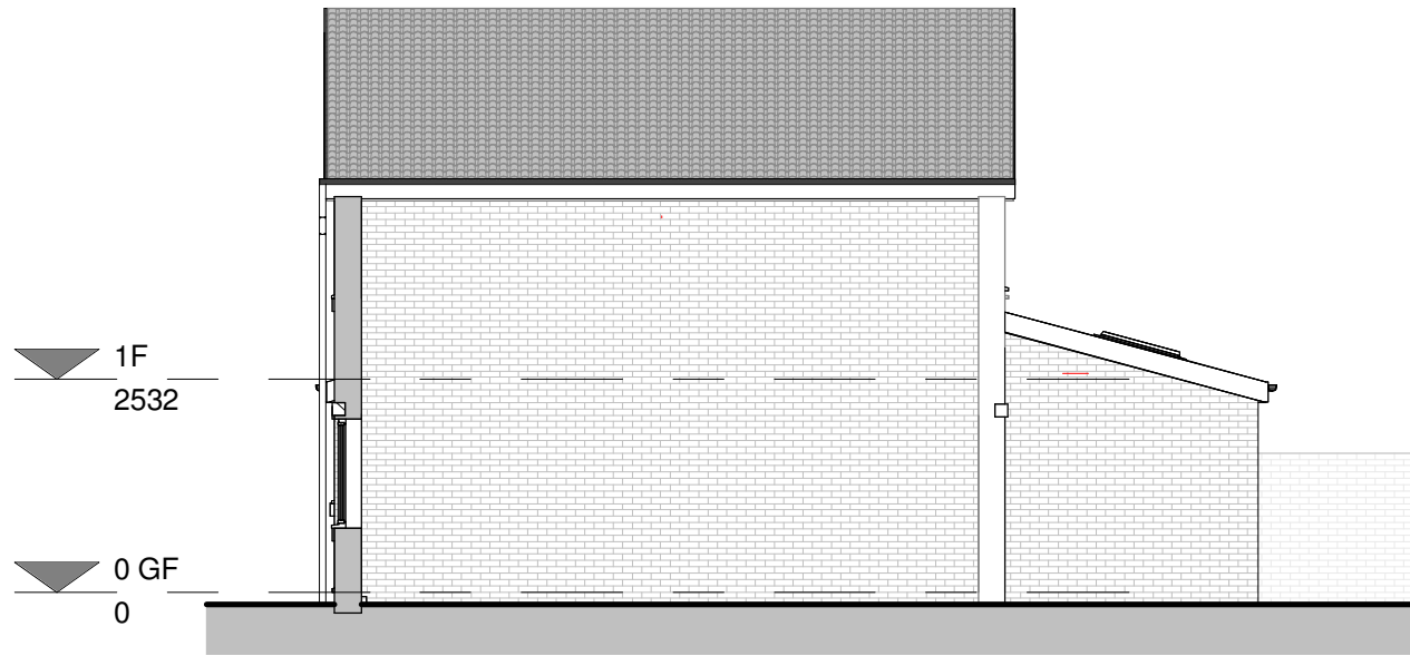
SIDE ELEVATION II
