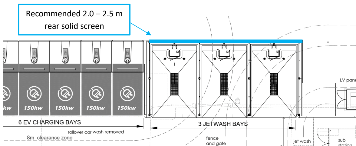
Figure 1 – Figure showing recommended 2.0 – 2.5 m acoustic barrier about rear of proposed jet wash bays.
