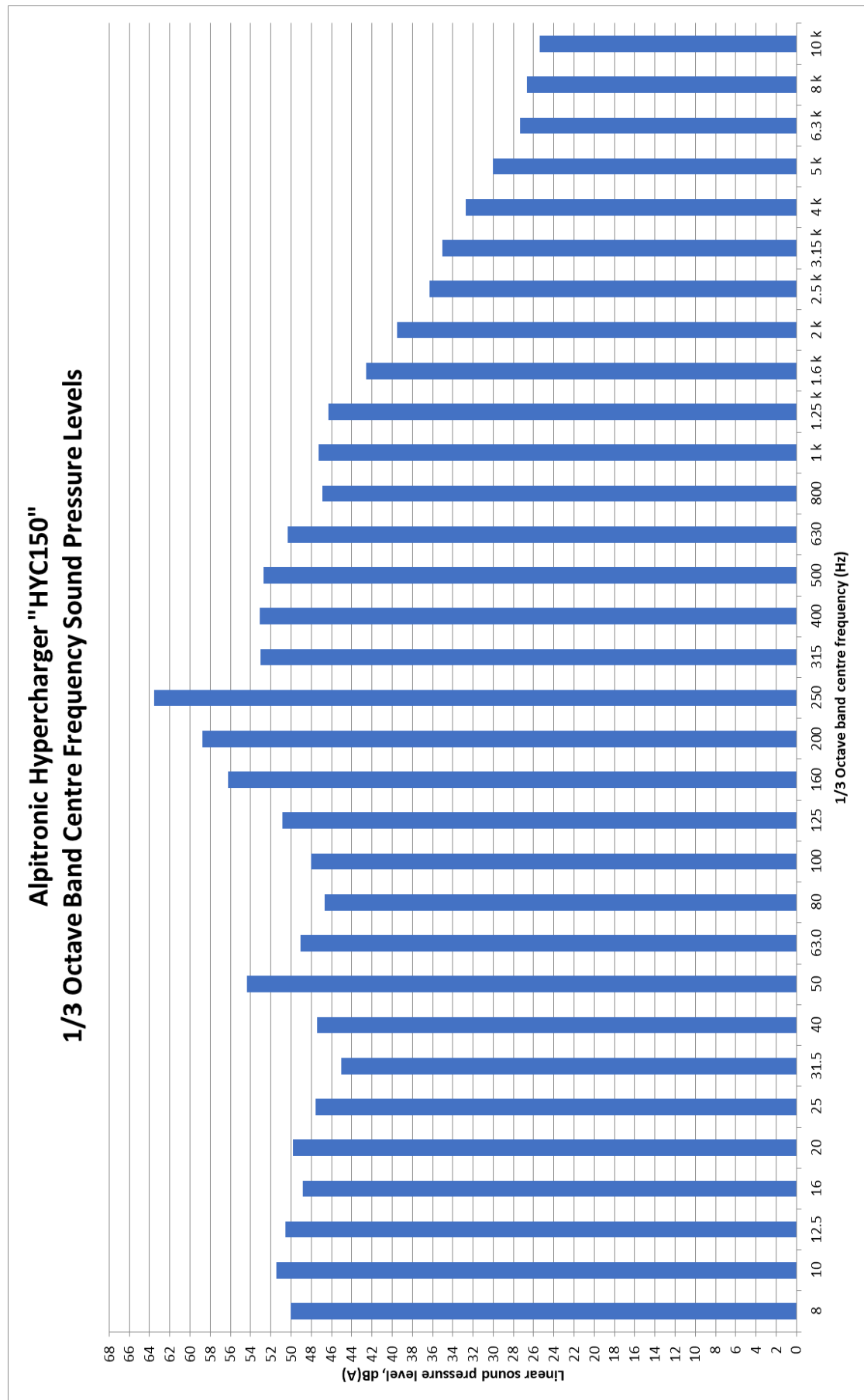
Figure D6 – Alpitronic Hypercharger (HYC150) Linear 1/3 Octave Band Spectral Results (average).
