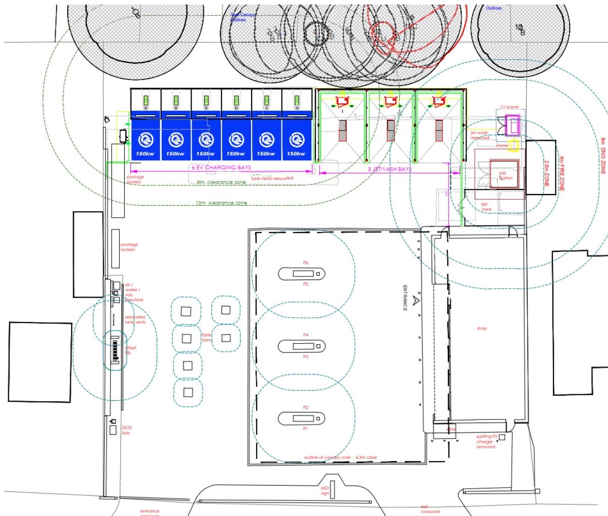
Figure C1 – Proposed development site plan.
