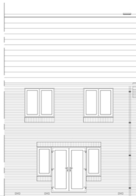
REAR ELEVATION - STANDARD
