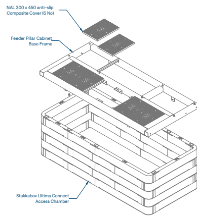
Exploded view feeder pillar omitted for clarity
