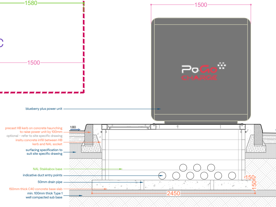
Front Sectional Elevation
