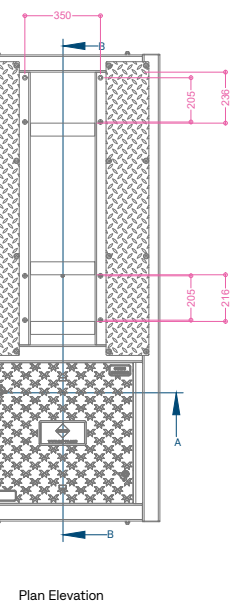
Plan Elevation
