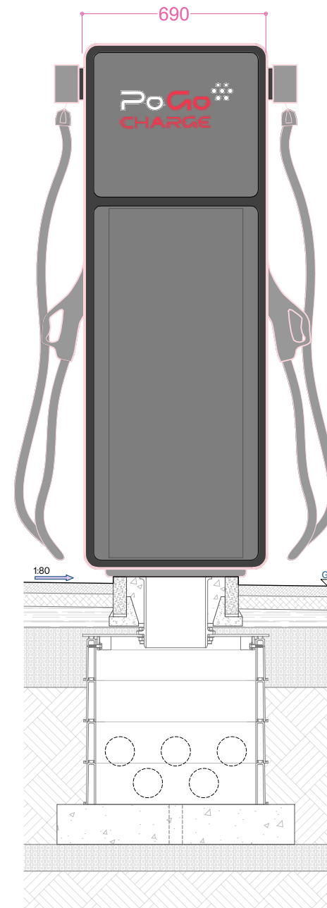
Rear Sectional Elevation
