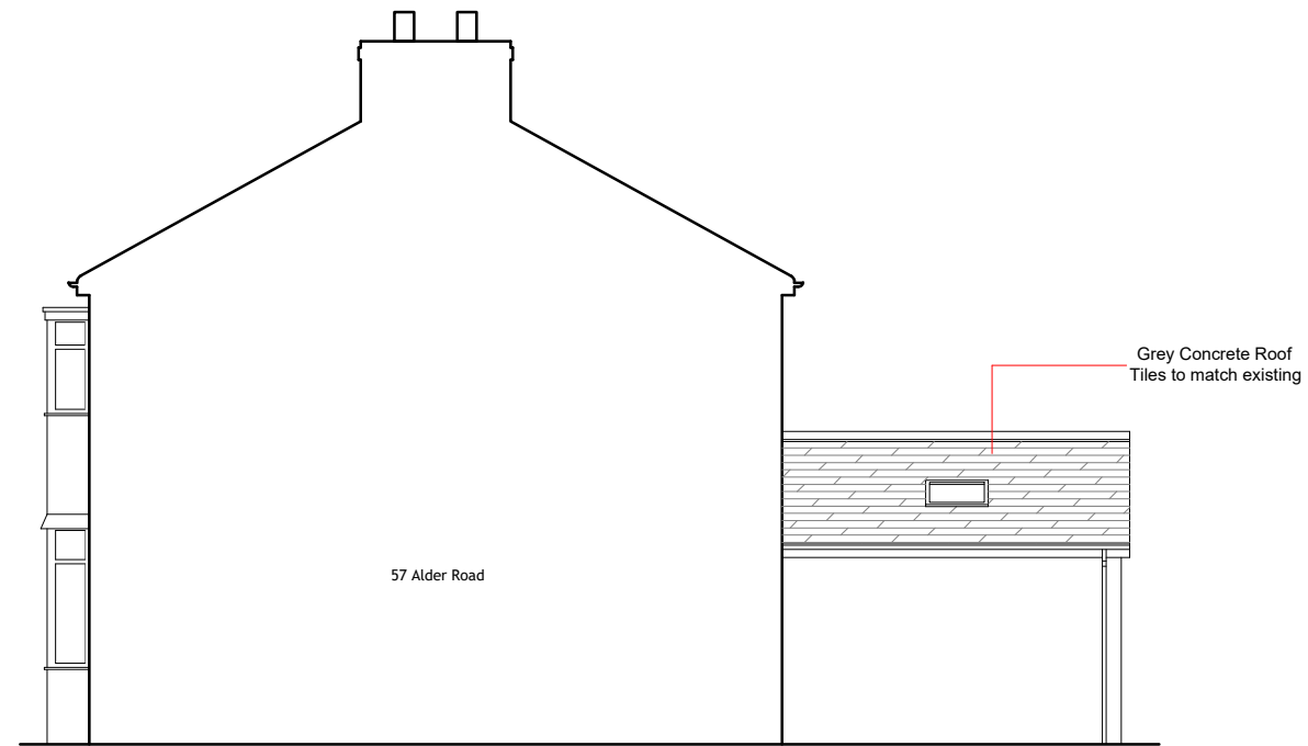
Proposed East Side Elevation
