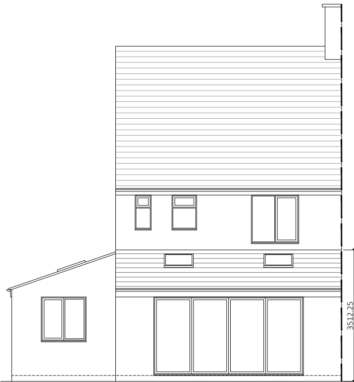
REAR ELEVATION
