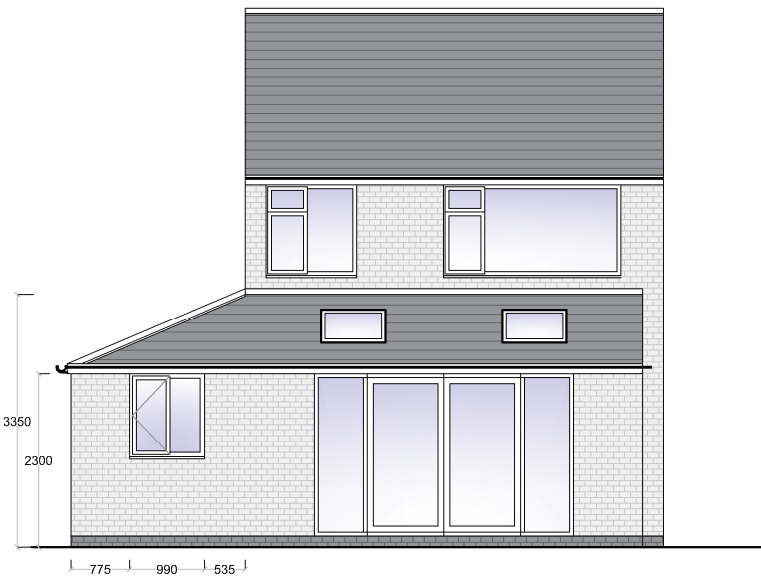
PROPOSED REAR ELEVATION (Scale 1:100) SCALE BAR - (mm) 500 1000 2000
