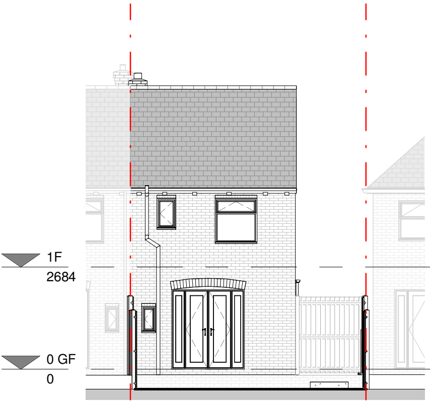
REAR ELEVATION
