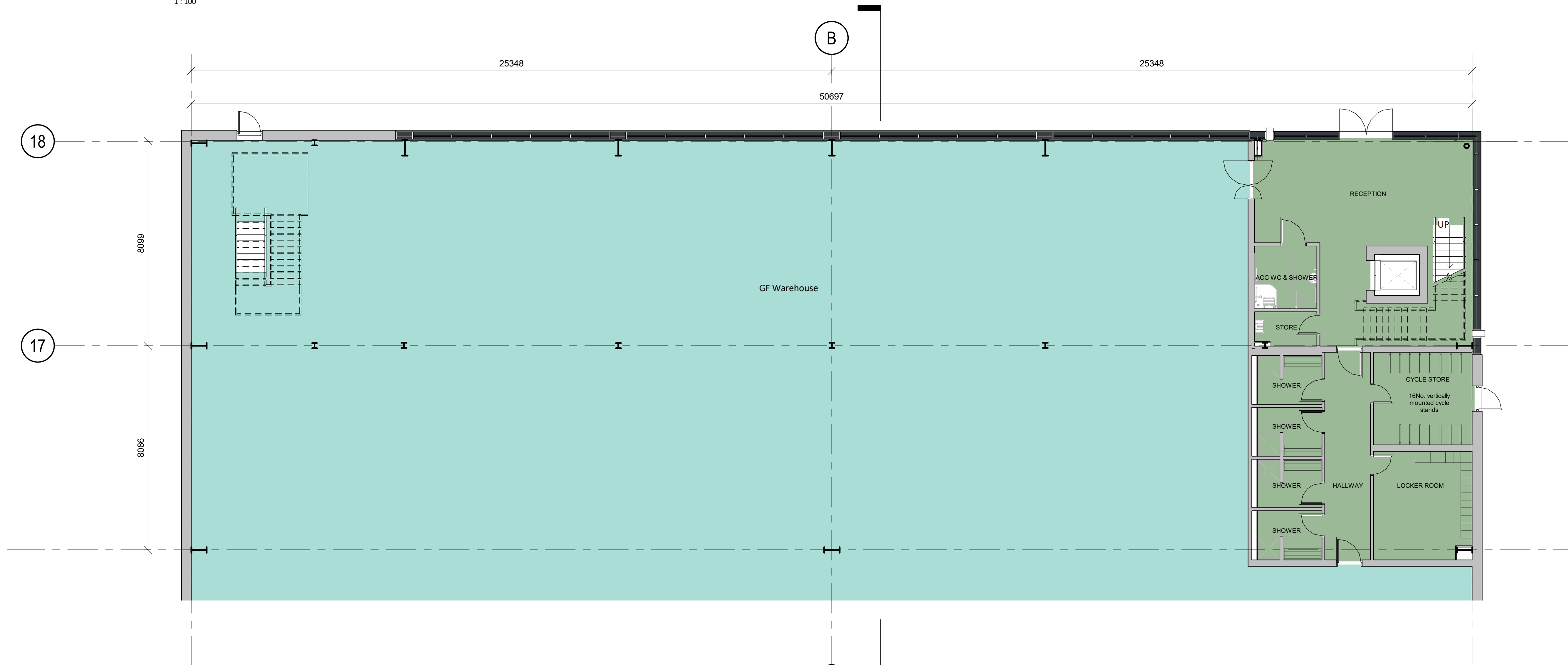
Ground Floor Office GA Plan 1 : 100
