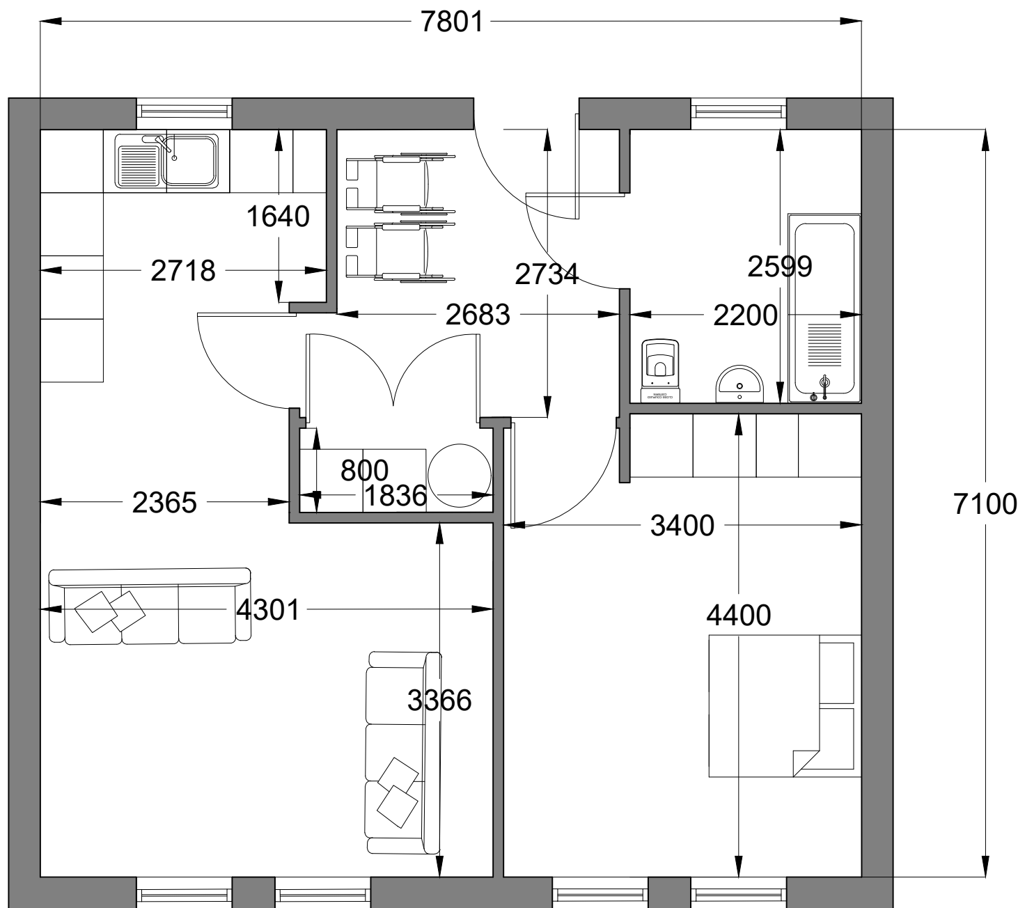
APT Type 3 (1 bed)
