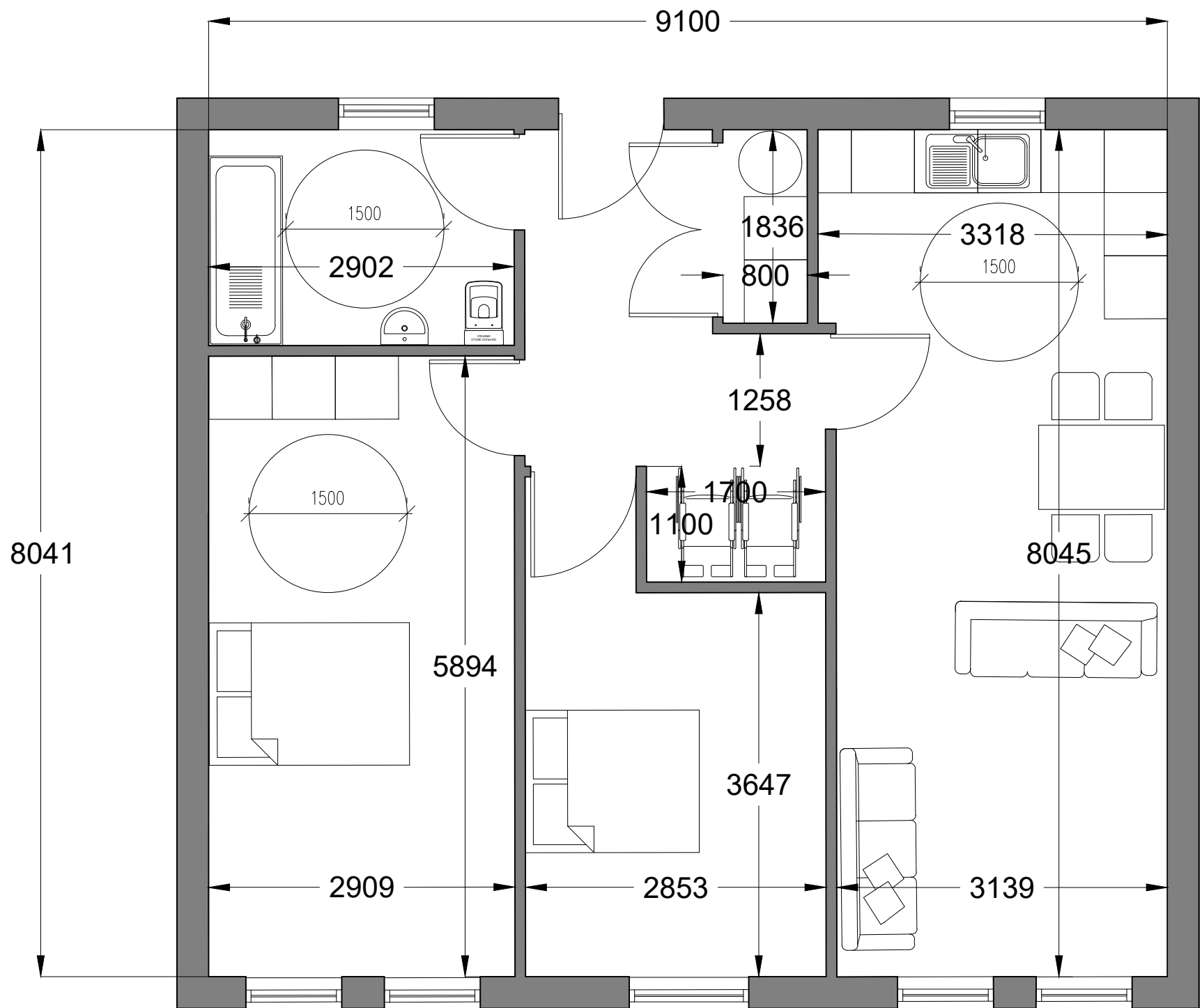
APT Type 2 (2 bed)
