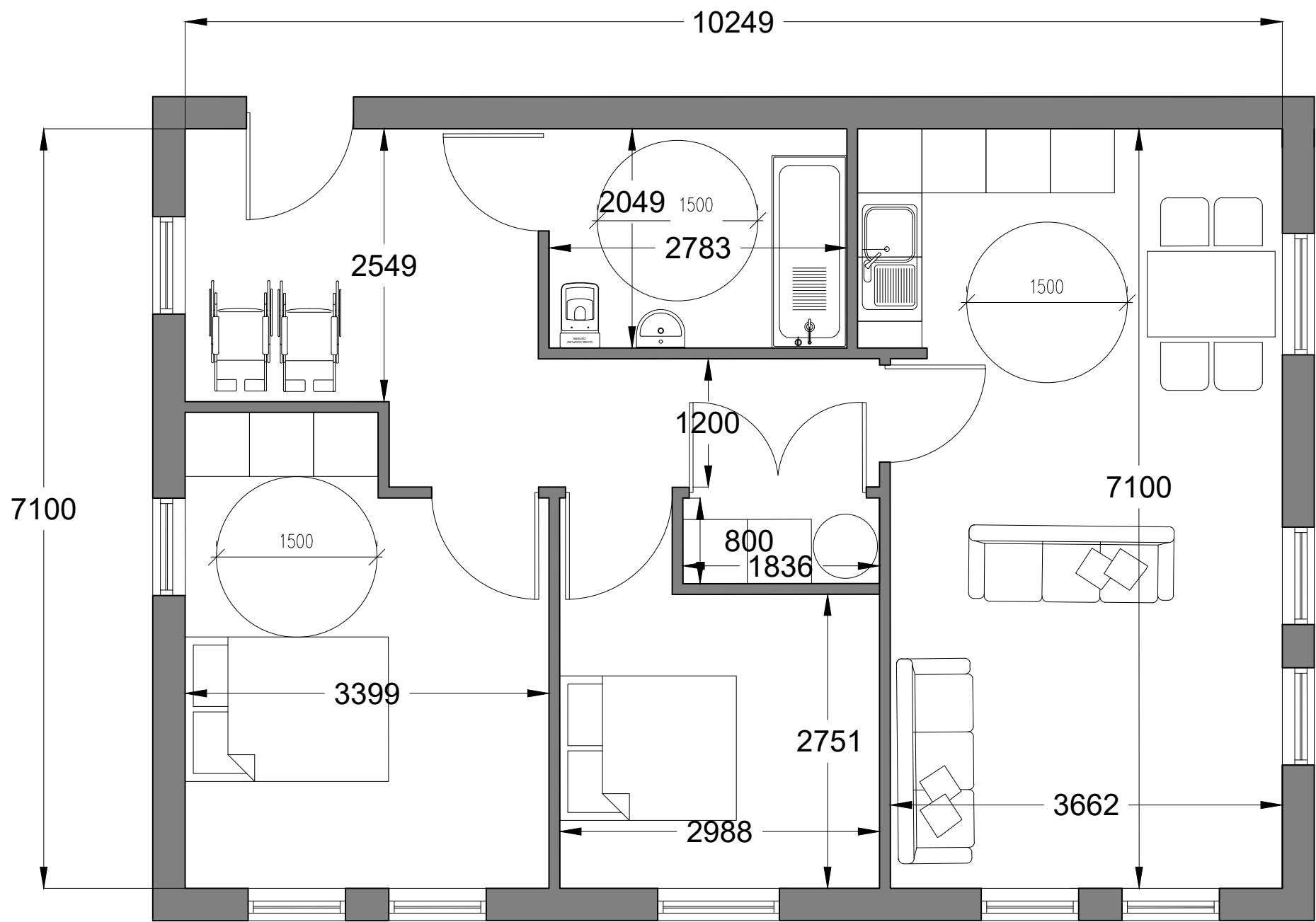
APT Type 1b (2 bed)
