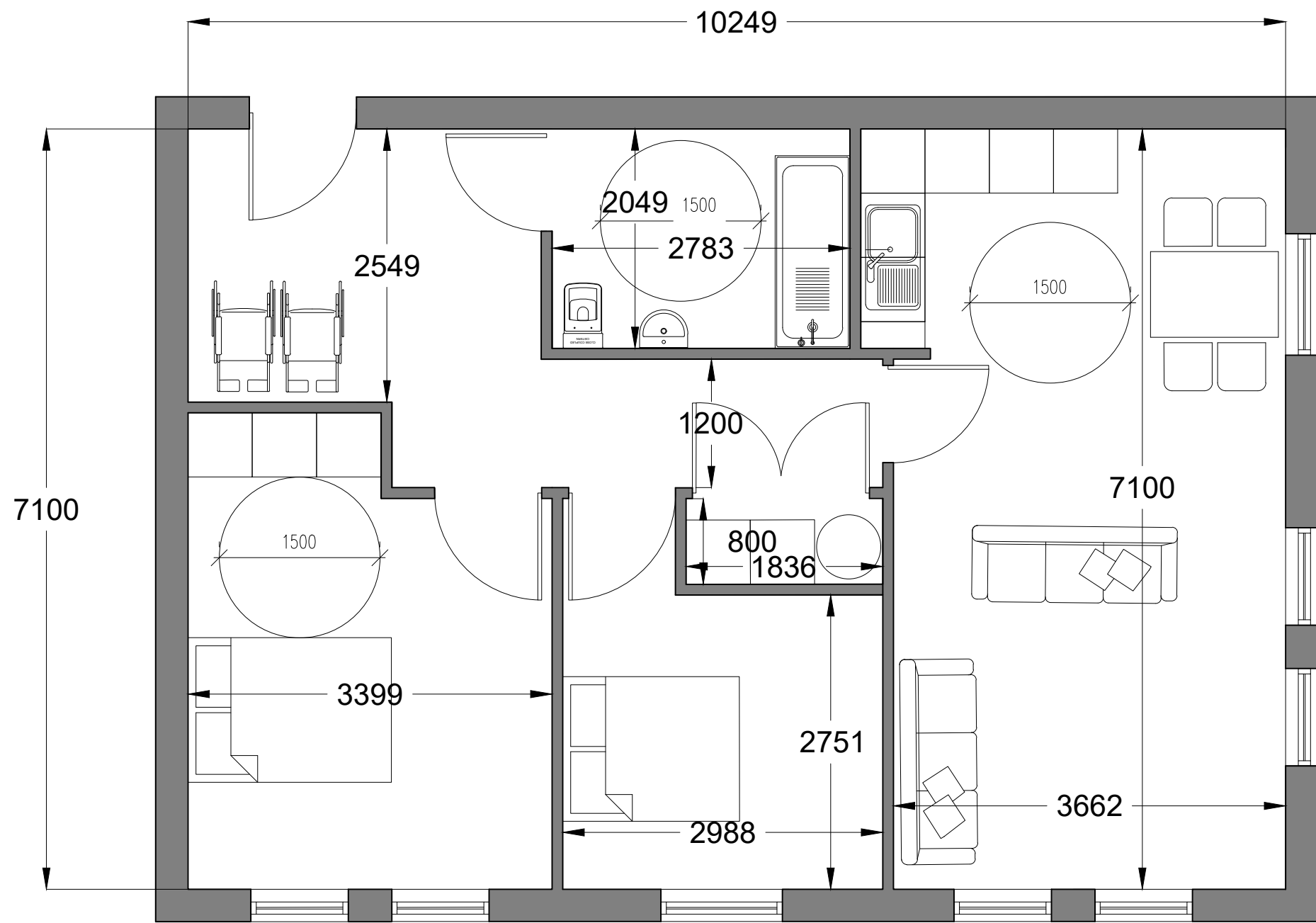
APT Type 1 (2 bed)
