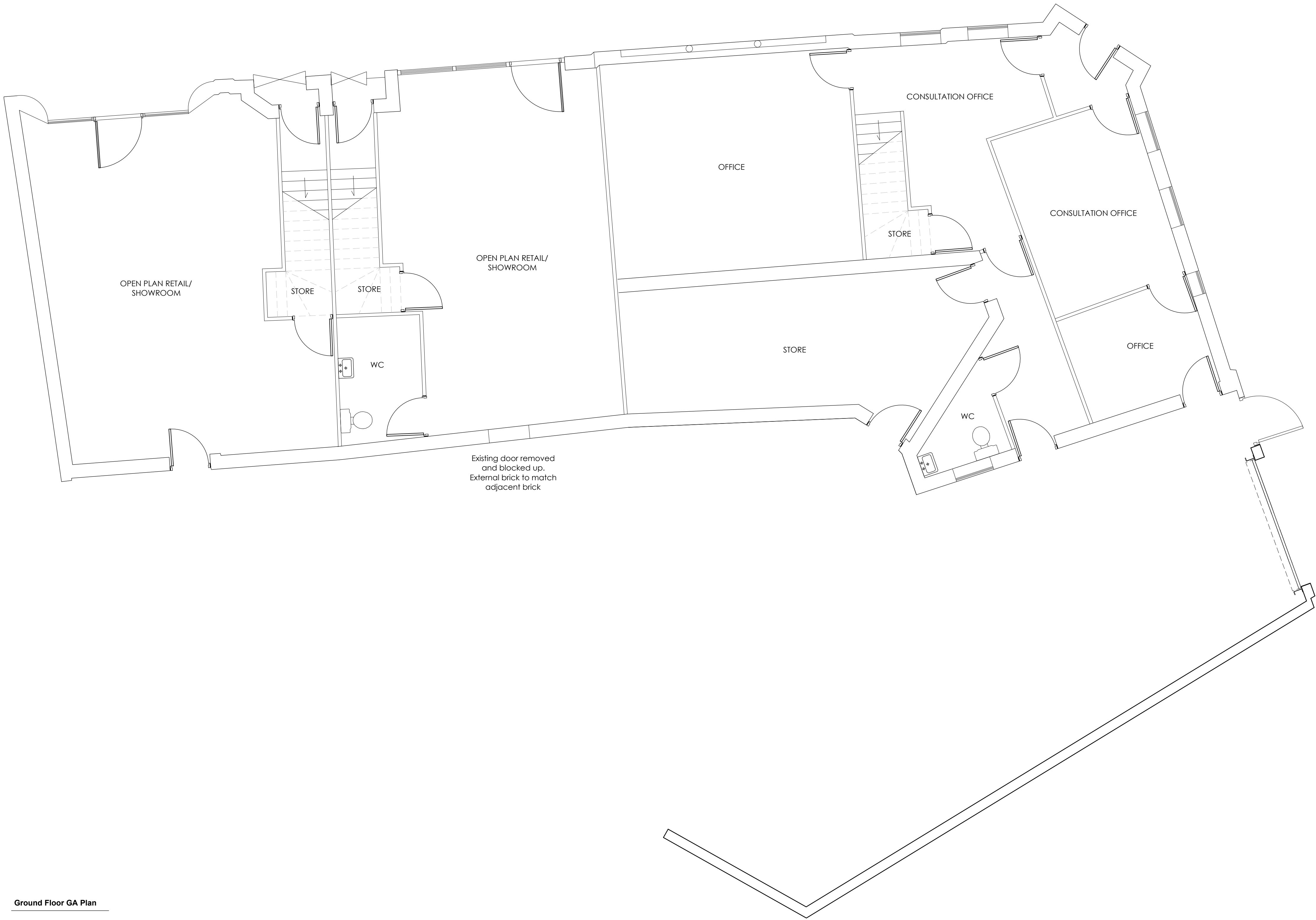
Ground Floor GA Plan
