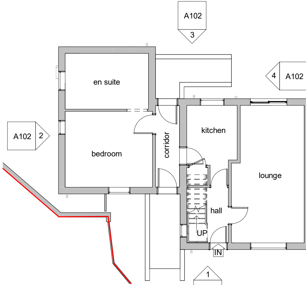
1 L0 Plan as Existing 1 : 100
