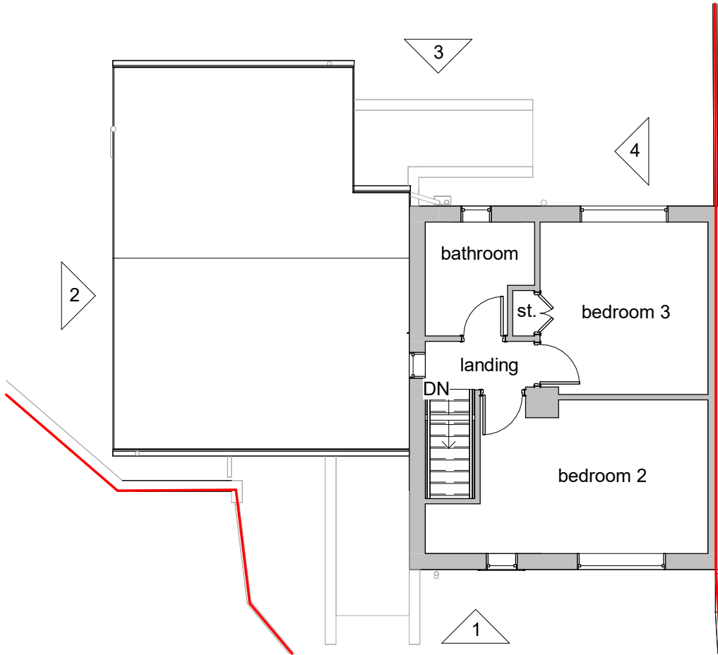
2 L1 Plan as Existing 1 : 100
