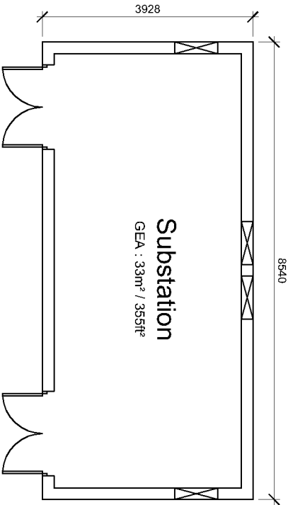
Floor Plan
