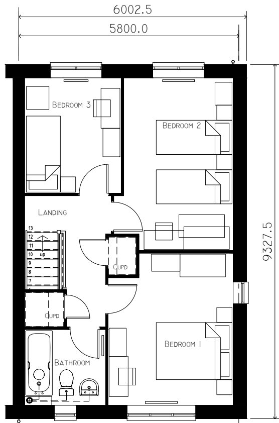
FIRST FLOOR PLAN GFA 47.42M2 (46.58M2)
