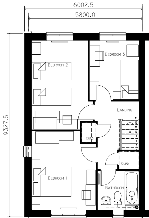
FIRST FLOOR PLAN GFA 47.42M2 (46.58M2)
