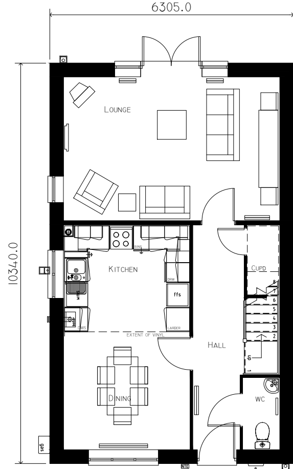
GROUND FLOOR PLAN GFA 53.96M2 (53.05M2)
