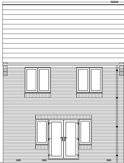
REAR ELEVATION - STANDARD
