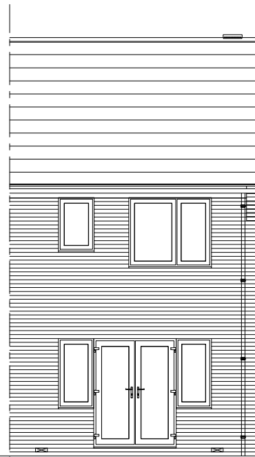
REAR ELEVATION
