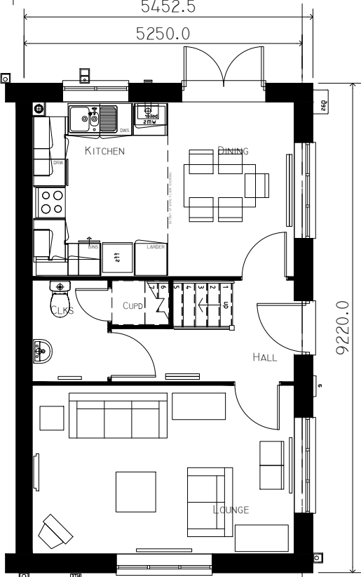
GROUND FLOOR PLAN GFA 42.15M2 (41.34M2)
