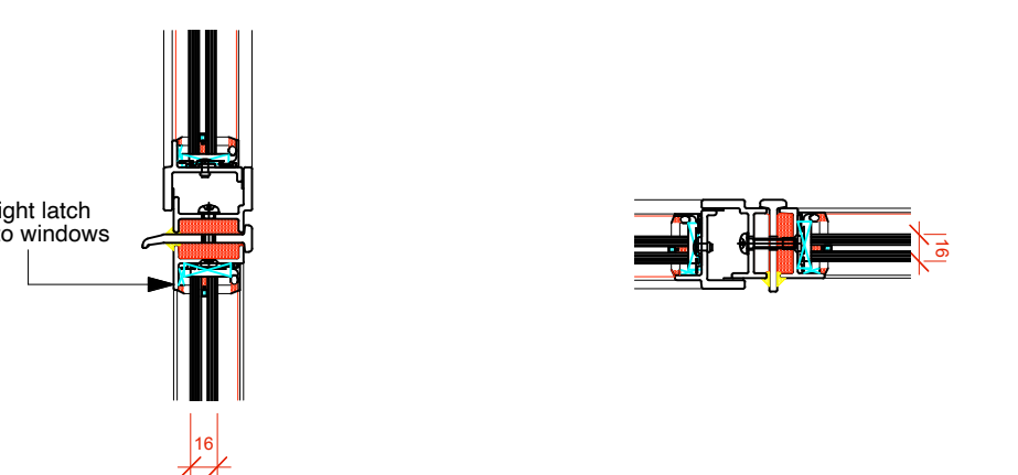
Detail 15 (scale 1:5)
