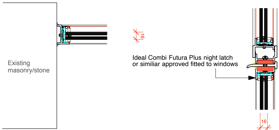
Detail 13 (scale 1:5)
