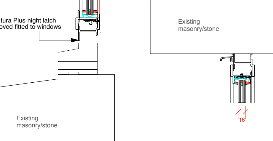
Detail 18 (scale 1:5)
