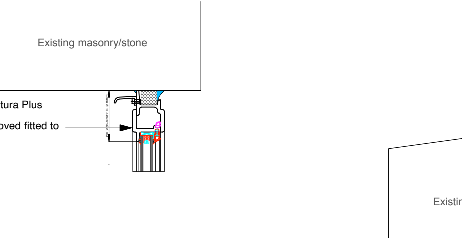
Detail 10 (scale 1:5)
