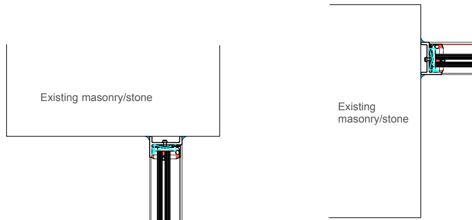
Detail 11 (scale 1:5)
