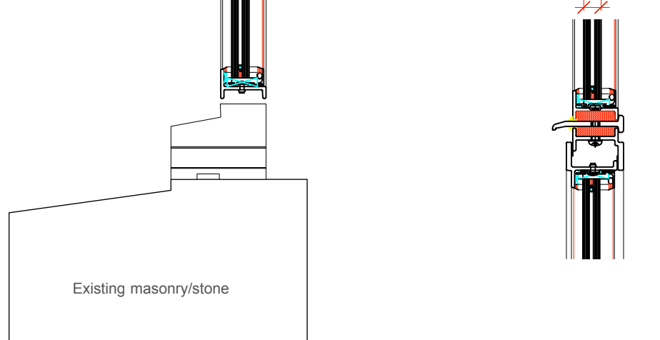
Detail 12 (scale 1:5)
