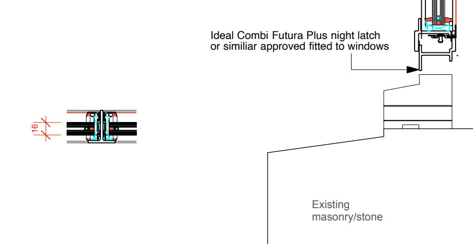
Detail 16 (scale 1:5)
