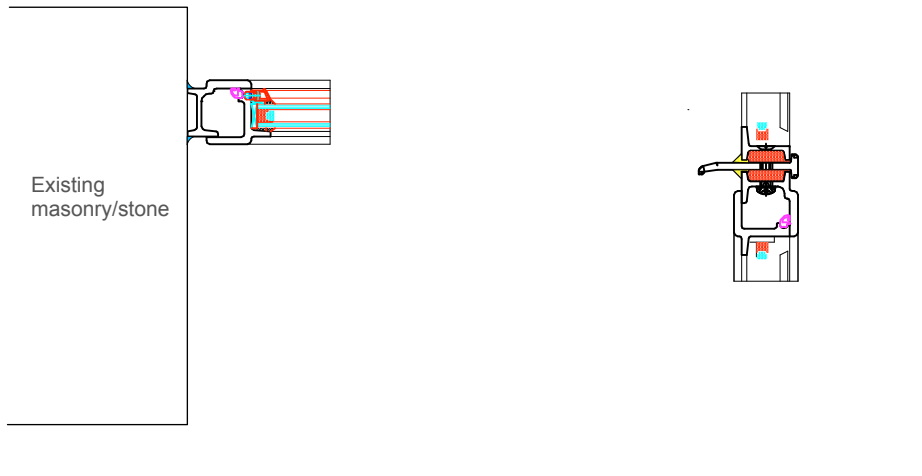
Detail 04 (scale 1:5)
