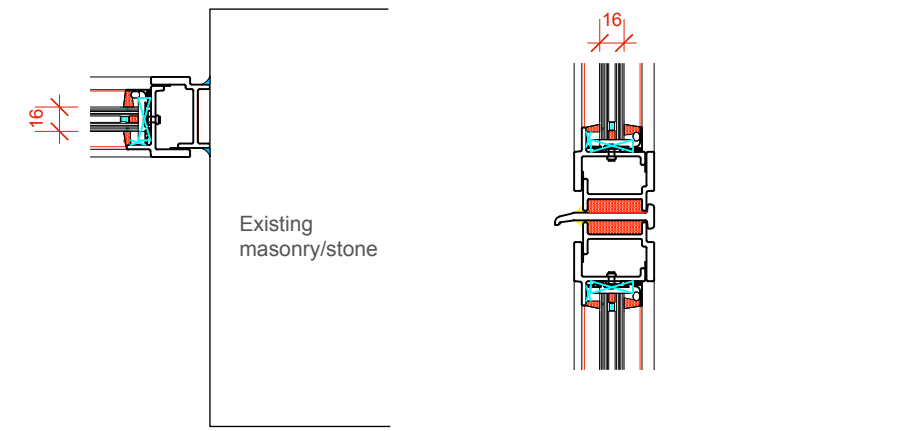
Detail 19 (scale 1:5)
