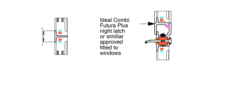
Detail 05 (scale 1:5)
