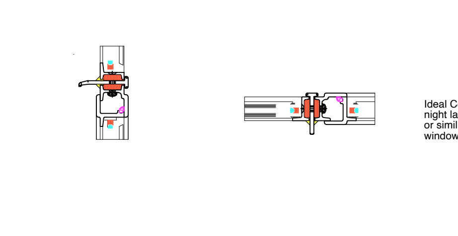
Detail 06 (scale 1:5)
