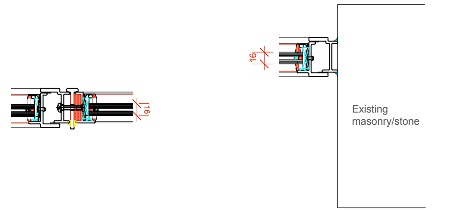
Detail 17 (scale 1:5)
