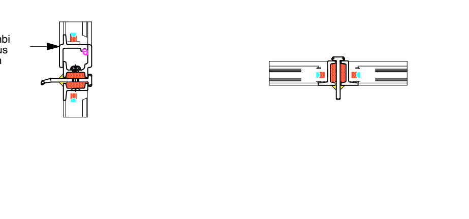
Detail 07 (scale 1:5)
