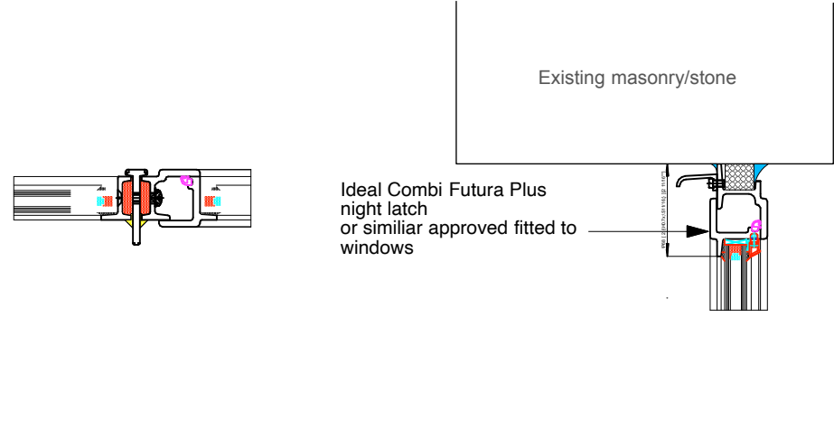
Detail 08 (scale 1:5)
