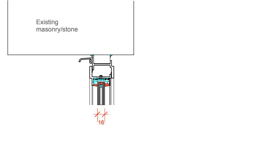
Detail 20 (scale 1:5)
