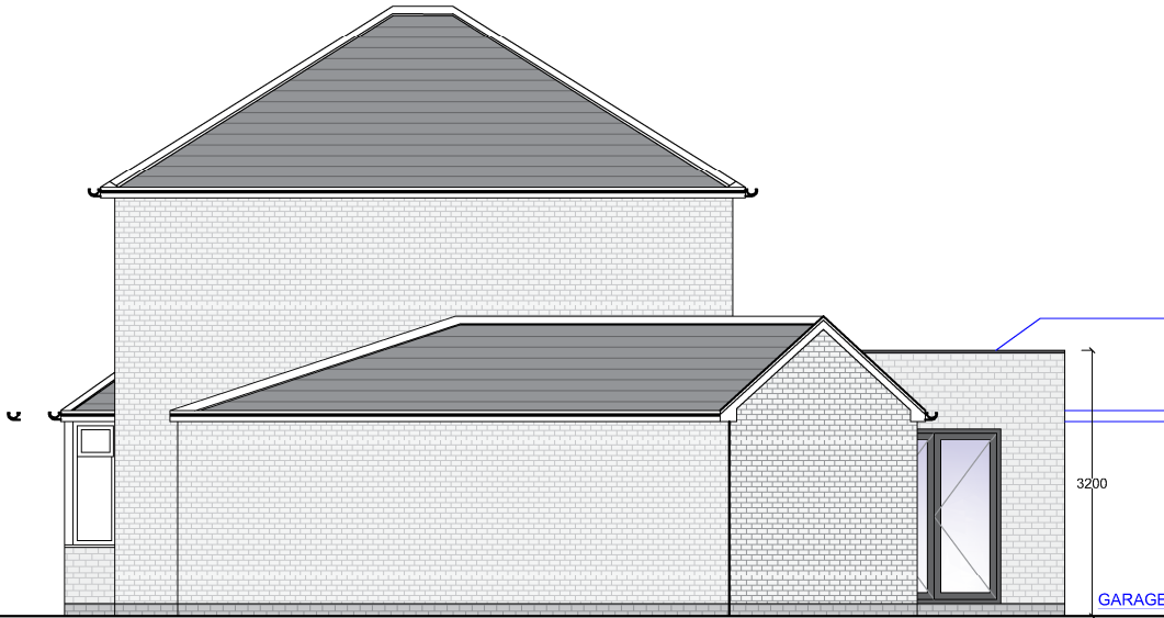
PROPOSED SIDE ELEVATION (Scale 1:100) SCALE BAR - (mm) 500 1000 2000
