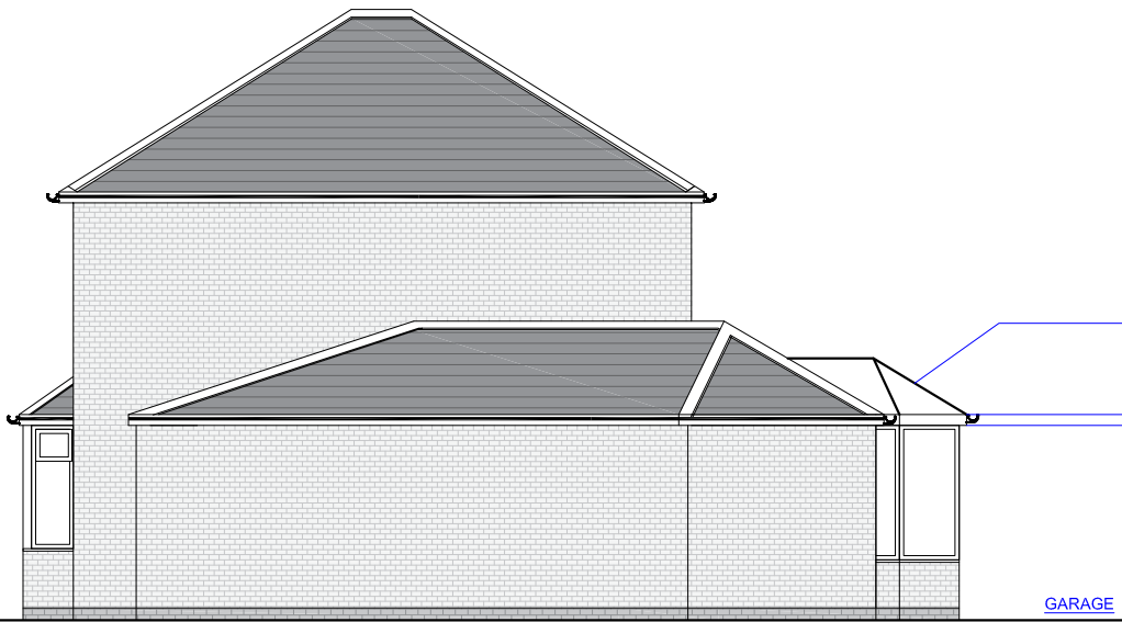
EXISTING SIDE ELEVATION (Scale 1:100) SCALE BAR - (mm) 500 1000 2000
