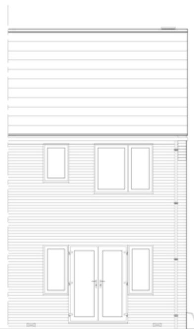
REAR ELEVATION
