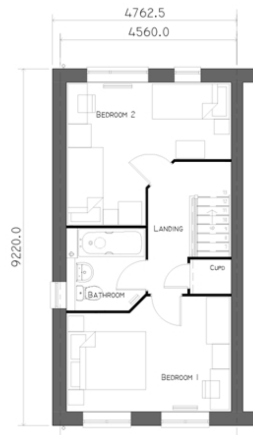
FIRST FLOOR PLAN GFA 36.27M 2 (35.51M 2 )
