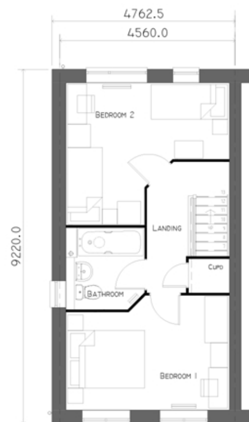
FIRST FLOOR PLAN GFA 36.27M 2 (35.51M 2 )
