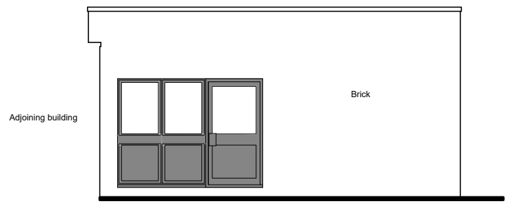
08 SOUTH WEST elevation
