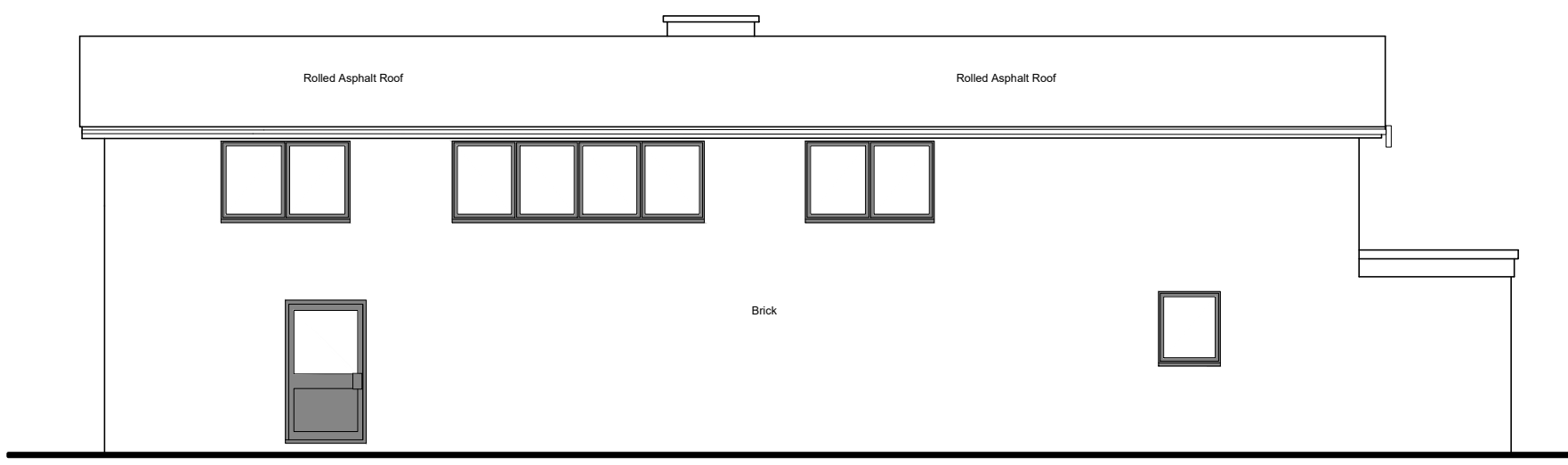
10 SOUTH EAST elevation
