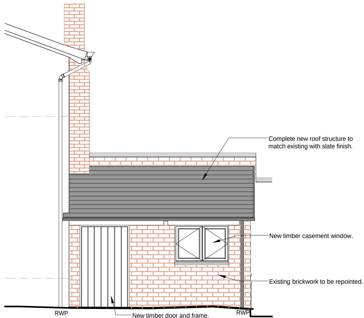
FRONT ELEVATION - 1:50
