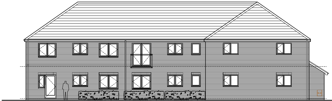
East Elevation (facing park)
